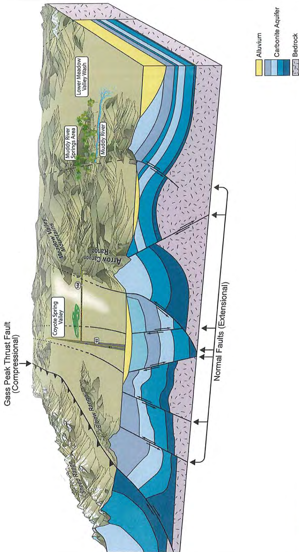
Conceptual Geologic Cross-Section of Coyote Spring Valley and Muddy River Springs Area
