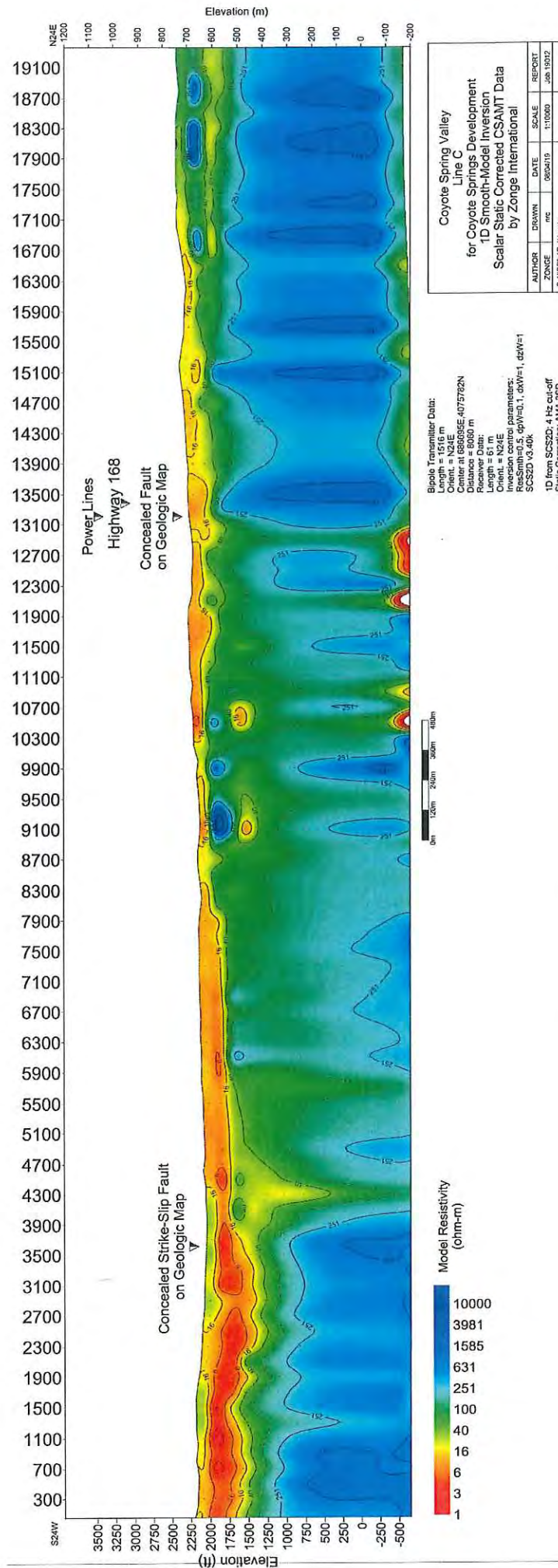
APRIL 2019 CSAMT RESULTS RESISTIVITY CROSS-SECTION LINE C
