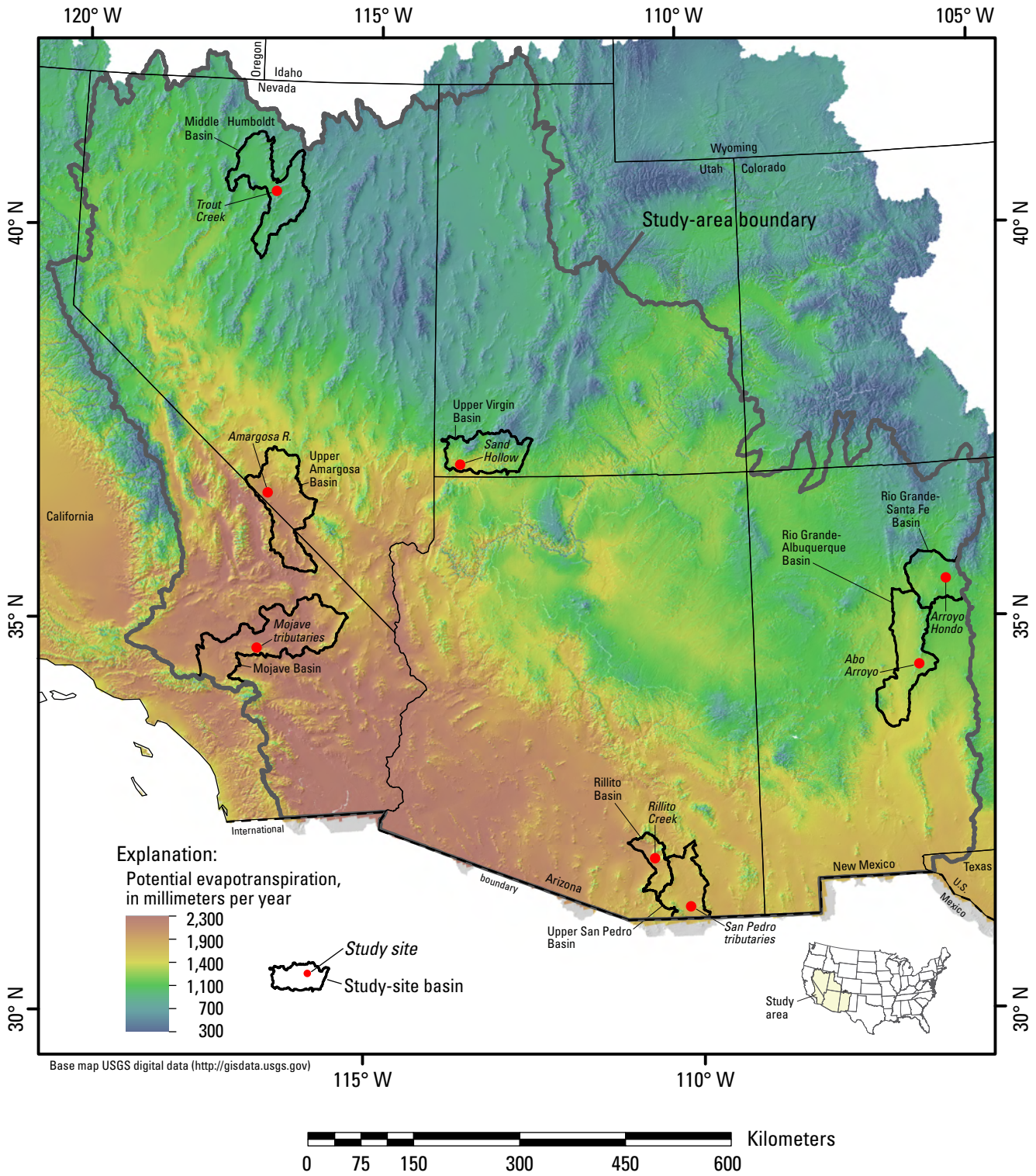
Figure 7. Average annual potential evapotranspiration in the modeled arid and semiarid southwestern United States.
