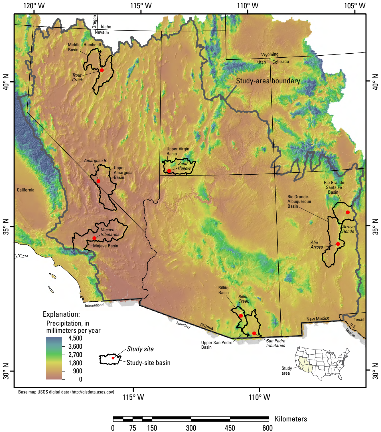
Figure 2. Average annual precipitation for 1971–2000 within the modeled arid and semiarid southwestern U.S. study area, calculated from monthly Precipitation-elevation Regression on Independent Slopes Method (PRISM) data (Daly and others, 2004).
