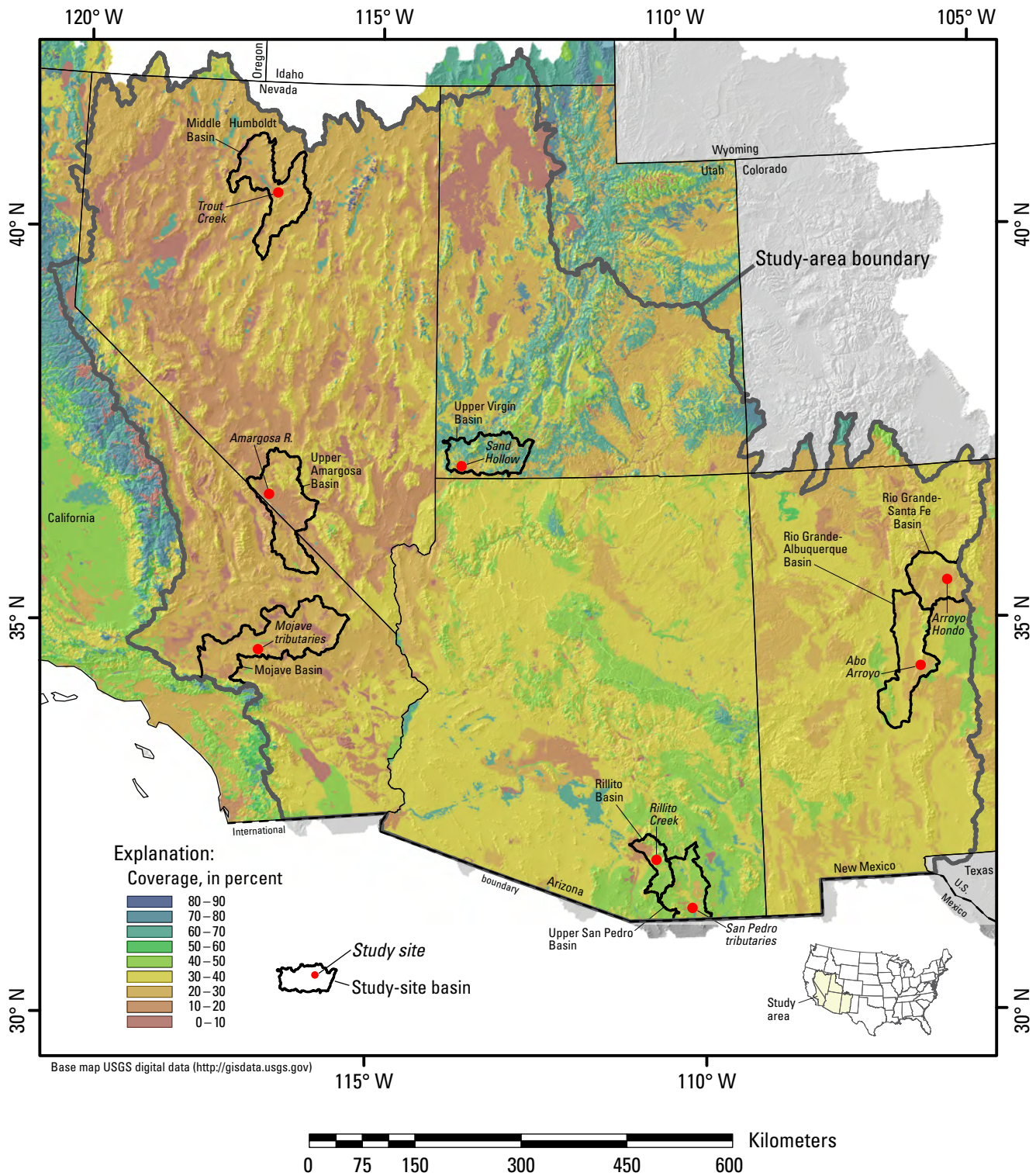
Figure 8. Percentage of area covered by vegetation in the modeled arid and semiarid southwestern United States.
