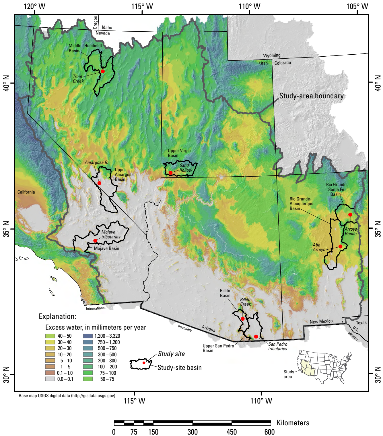
Figure 3. Estimates of annual excess water within the modeled arid and semiarid southwestern United States study area, calculated as the summed values of average monthly precipitation minus average monthly potential evapotranspiration. Texas, Wyoming, and portions of Colorado outside the study area were not included in the analysis.
