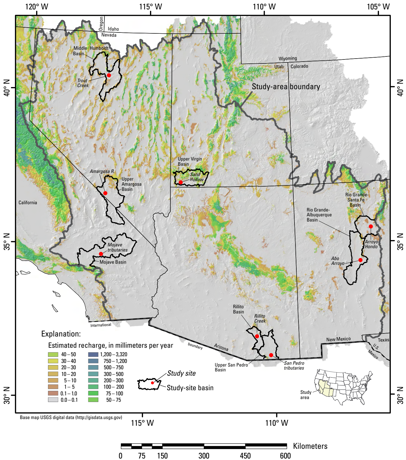
Figure 11. Average annual ground-water recharge within the modeled arid and semiarid southwestern United States study area, calculated with the Basin Characterization Model as in-place recharge plus 15 percent of runoff. Calculations used 30 years of average monthly precipitation and other dynamic input data from 1971–2000. Portions of Colorado outside the study area, Texas, and Wyoming were not modeled.
