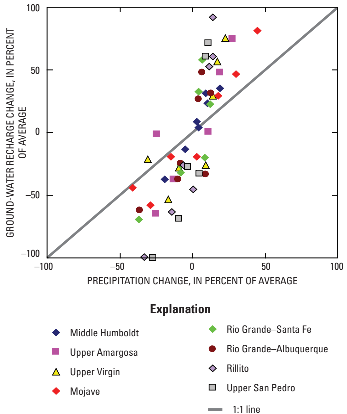
Figure 15. Change in ground-water recharge with change in precipitation, relative to respective 1971–2000 averages, for the eight basins containing recharge study sites. Different points for each basin represent varying combinations of climatic conditions as manifested in the El Niño-Southern Oscillation and Pacific Decadal Oscillation indices during 1941–2004. Ground-water recharge is estimated by using the Basin Characterization Model and assumes in-place recharge plus 15 percent of runoff.
