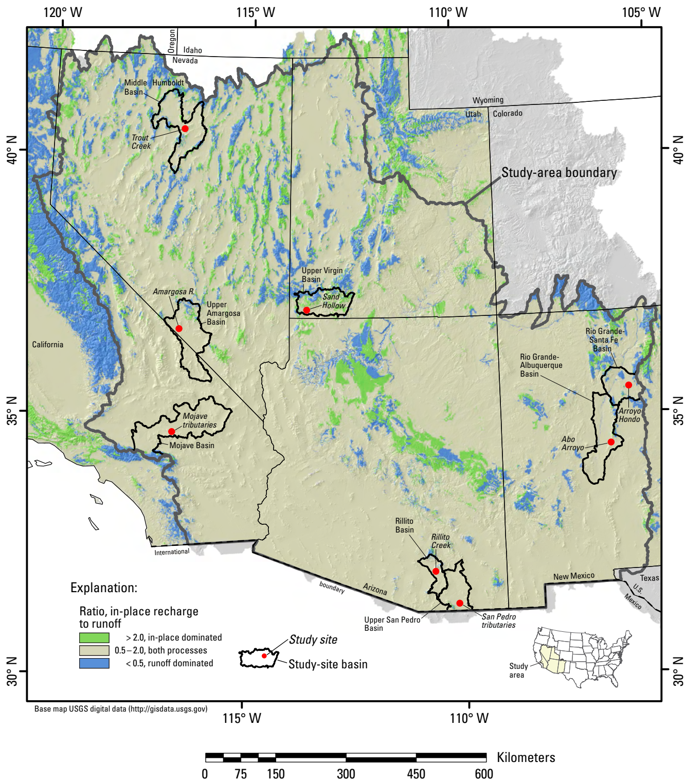
Figure 13. Areas within the modeled arid and semiarid southwestern U.S. study area, where runoff or in-place recharge is dominant, or where runoff and in-place recharge are nearly equal.
