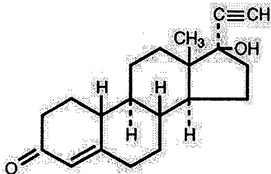
NORETHINDRONE
