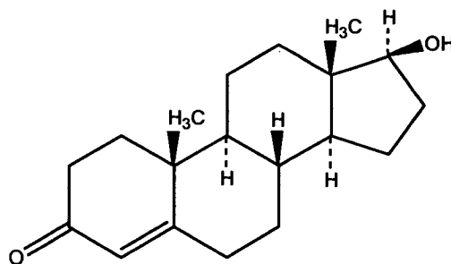
Testosterone
